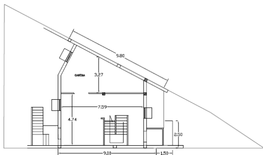
PIANO INTERRATO
